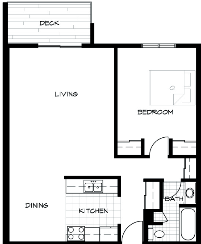
FLOOR PLAN - TYPICAL 1 BEDROOM
